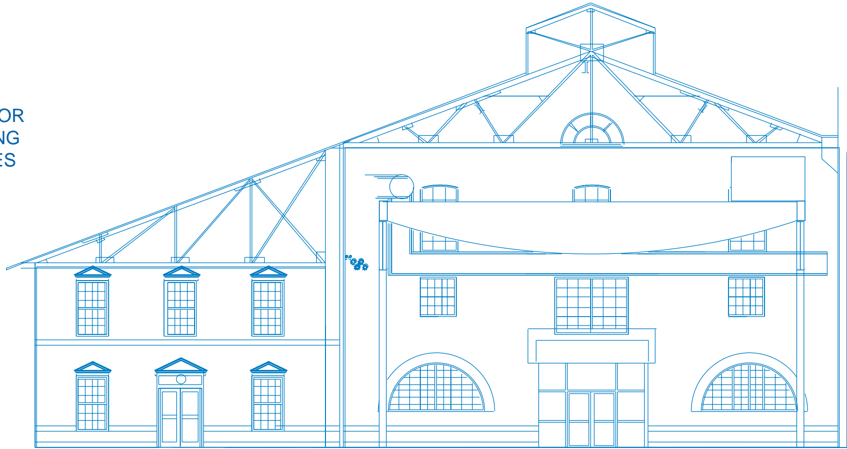
EAST WALL ELEVATION
